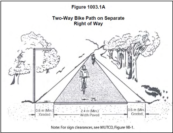
Source: Caltrans Highway Design Manual
