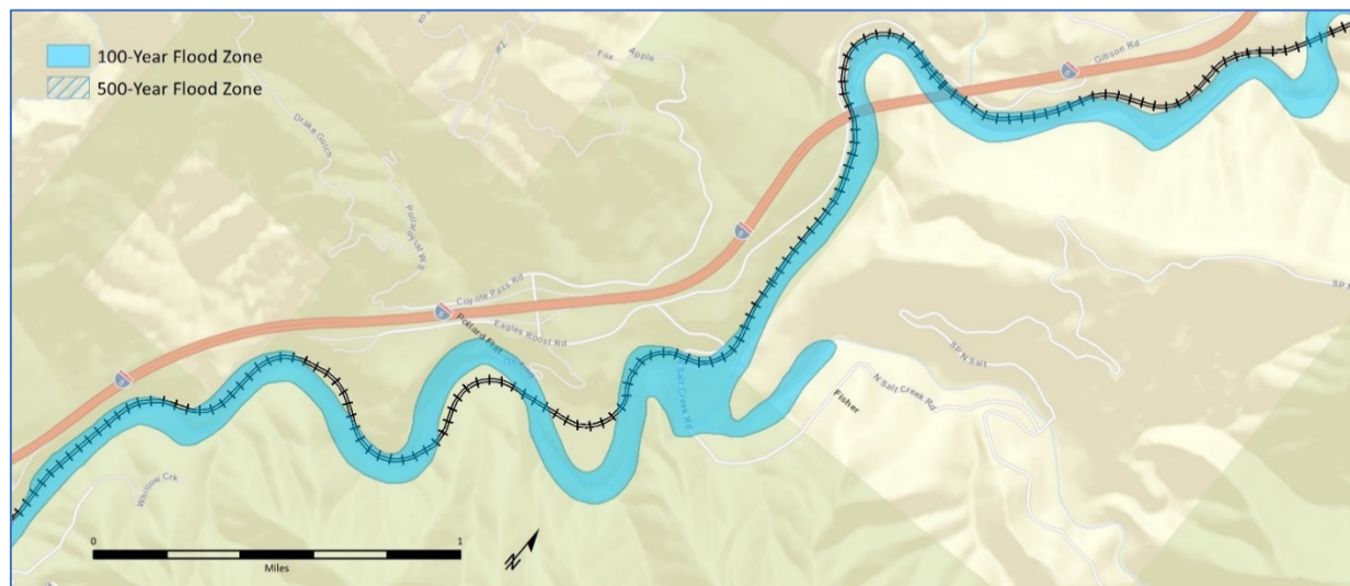
Figure 71. Flooding exposure of the Union Pacific Railroad in the Sacramento River Canyon, near Pollard
