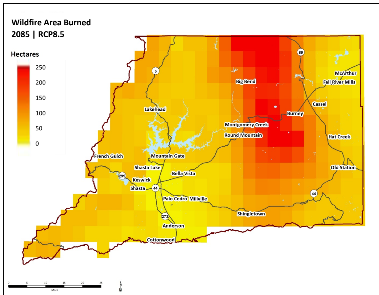
Figure 43. Average annual area burned in 2085, RCP8.5.
