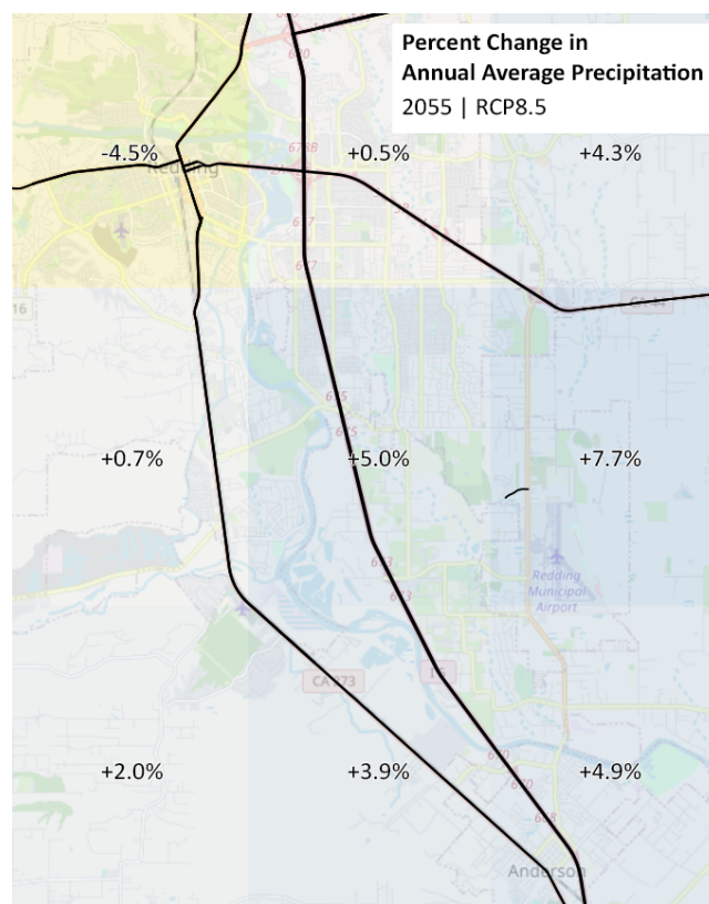
Figure 14. Detail of projected change in annual average precipitation in the Redding - Anderson area.
