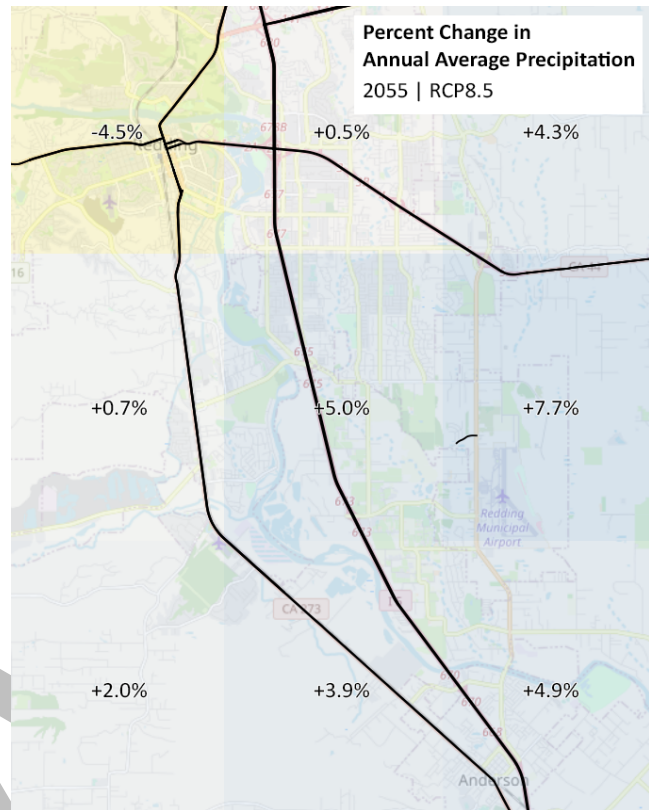
Figure 14. Detail of projected change in annual average precipitation in the Redding - Anderson area.
