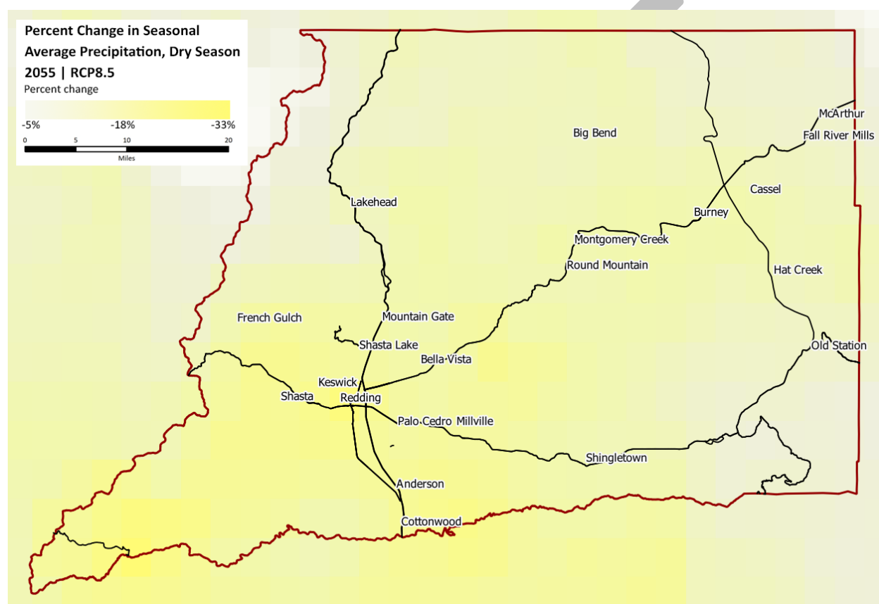
Figure 17. Percent change in dry season precipitation, 2055 RCP8.5.
