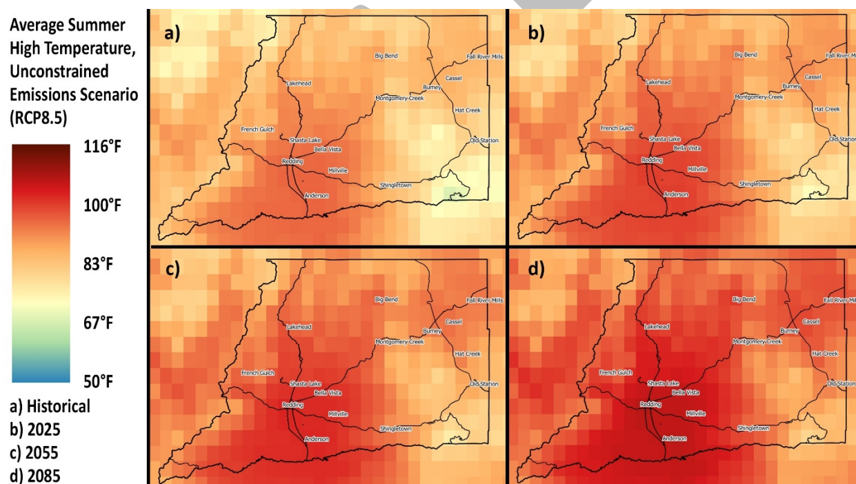
Figure 6. Projected changes to average summer high temperatures over the course of the 21 st century in an unconstrained emissions scenario. Average summer temperatures in Redding and the upper Sacramento River Valley are projected to exceed 100°F by midcentury in both the unconstrained and reduced emissions scenarios.
