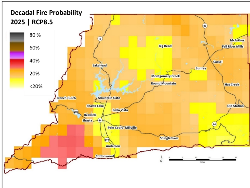
Figure 34. Decadal Fire Probability in 2025, RCP8.5.
