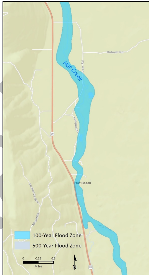
Figure 76. Flooding hazards associated with Hat Creek in the community of Hat Creek.
