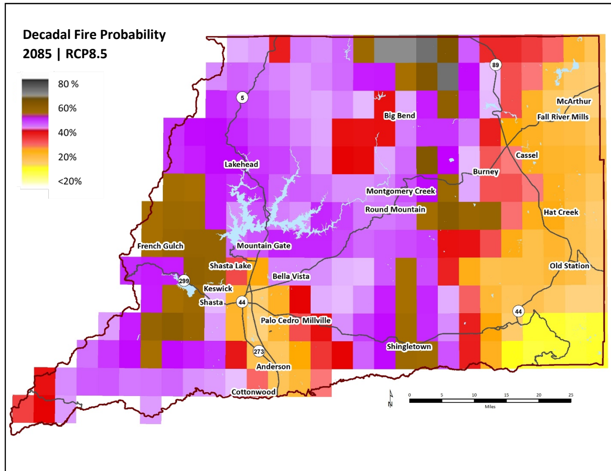
Figure 36. Decadal Fire Probability in 2085, RCP8.5.
