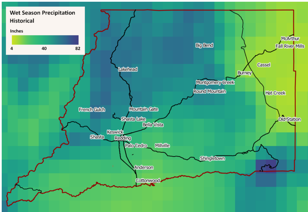
Figure 12. Historical average wet season precipitation in the Shasta Region.
