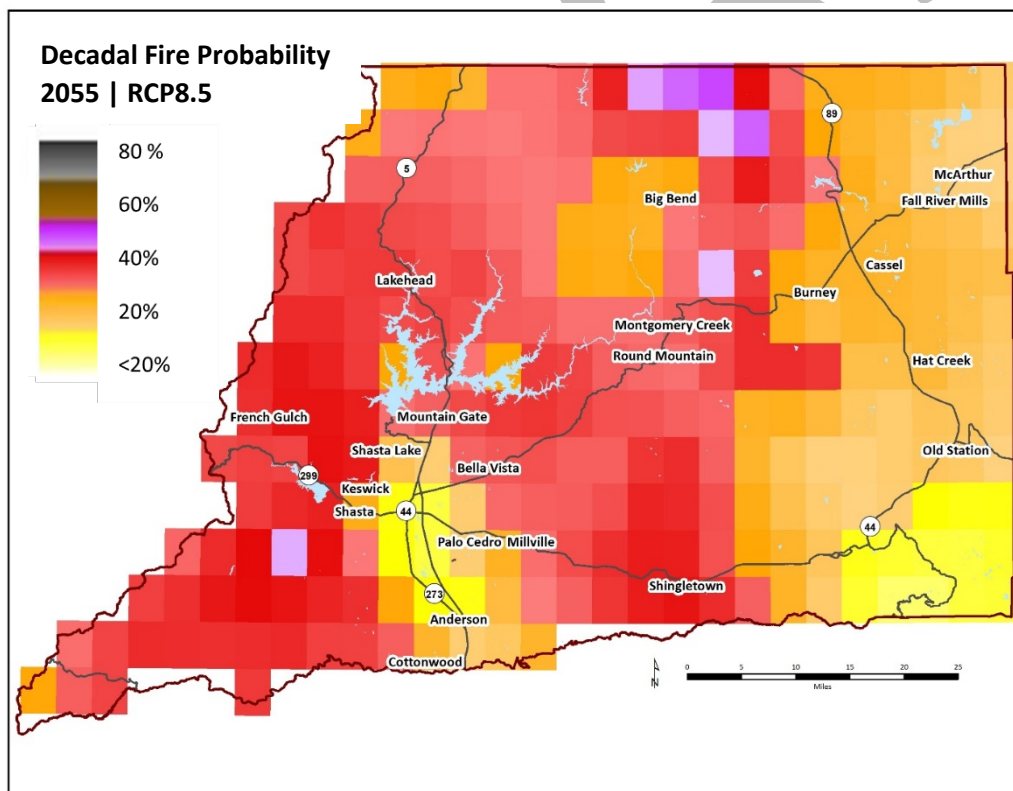
Figure 35. Decadal Fire Probability in 2055, RCP8.5.
