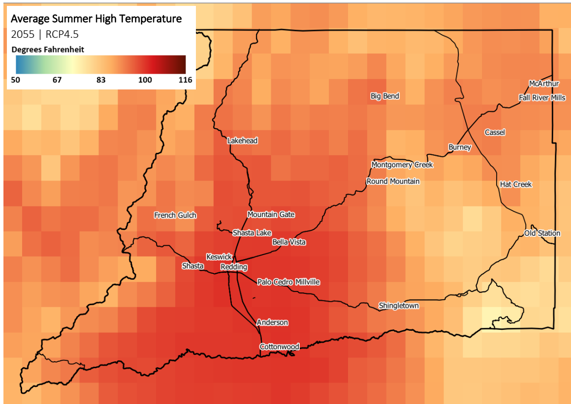
Figure 102. Average summer high temperatures, 2055, RCP4.5.
